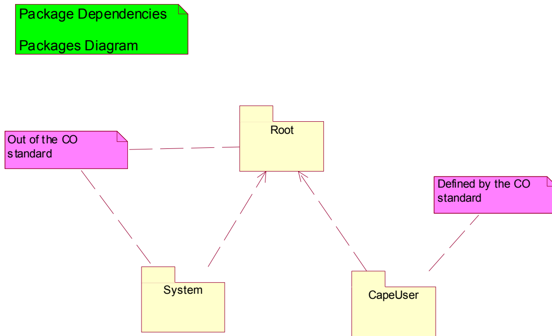
Figure 5 The package dependencies diagram
